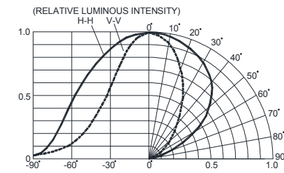
FIG.6 RED & BLUE&GREEN FAR FIELD PATTERN
