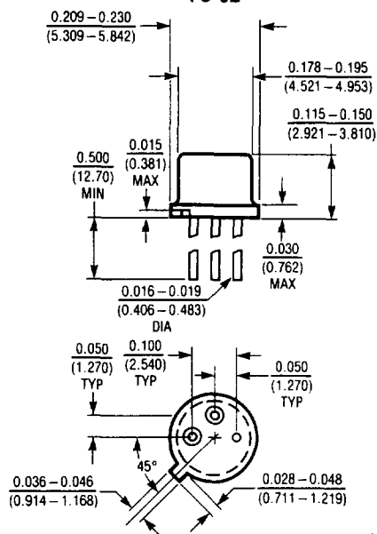
LT580 TO-52
