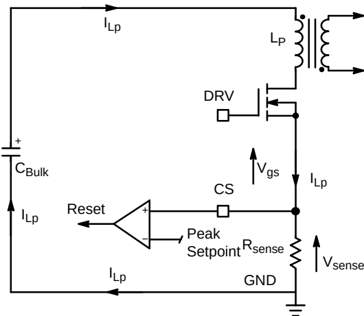
Figure 4. Positive Current-Sense Technique
