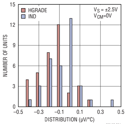
V_{OS} T_C (-40^{\circ}C \text{ to } 125^{\circ}C)
