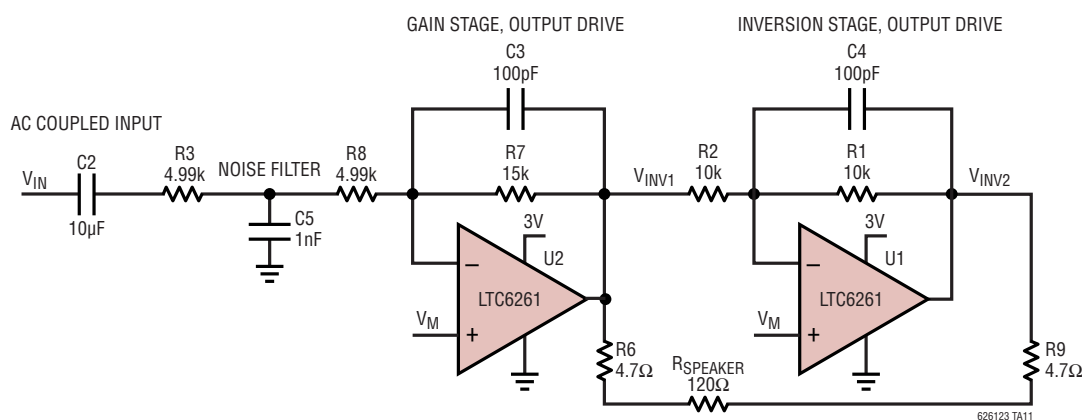
Audio Headphones Bridge Driver
