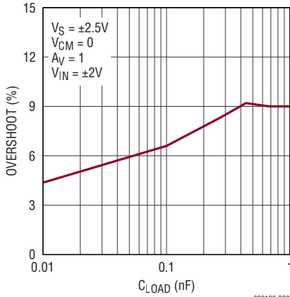
Capacitive Load Handling Overshoot vs Capacitive Load
