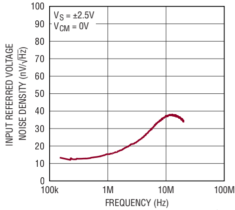
Noise Voltage Density vs Frequency
