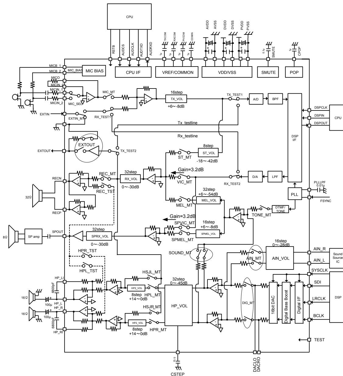
Fig.17 Recommended Circuit
