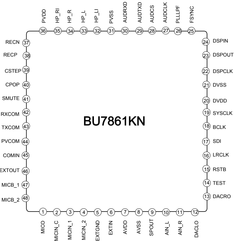
Fig.14 BU7861KN Pin Placement Diagram
