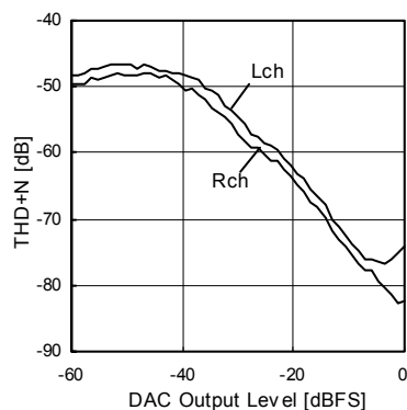
Fig.4 16bit D/A Converter Distortion @ 1kHz
