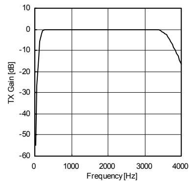
Fig.9 Voice CODEC TX Frequency Characteristics
