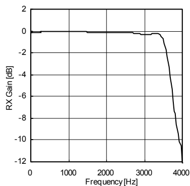
Fig.10 Voice CODEC RX Frequency Characteristics
