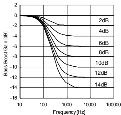
Fig.7 Bus Boost Frequency Characteristics
