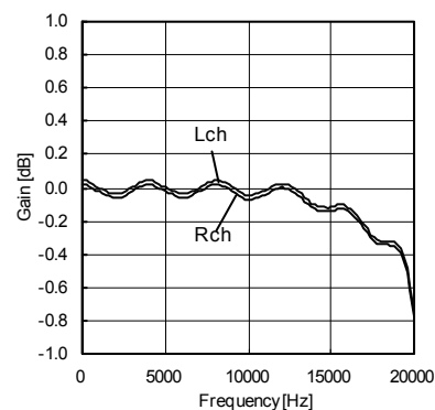
Fig.3 16bit D/A Converter Frequency characteristics @ 0dBFS
