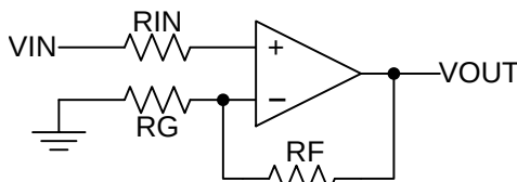
Figure 39. Layout Schematic
