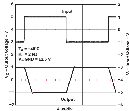
Figure 32. Large-Signal Inverting Response
