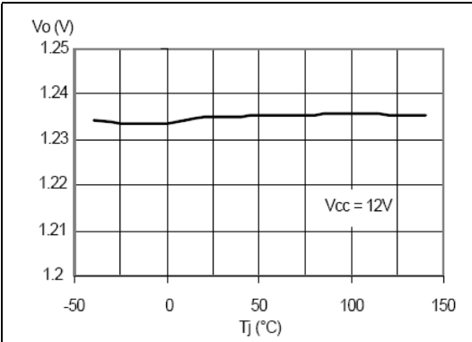
Figure 6. Output voltage vs junction temperature
