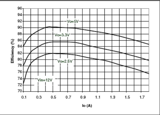
Figure 9. Efficiency vs output current
