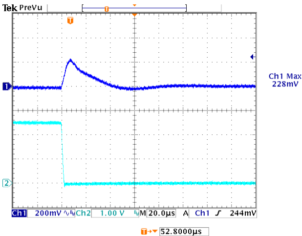
Figure 23: Typical Transient Response to Step Load Change at 2.5A/µS from 100% to 50% of I_o , max at 3.3Vin, 2.5Vout (Cout = 1µF ceramic, 10µF Tantalum)
