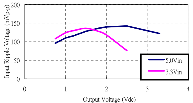
Figure 33: Input voltage ripple for various output models, IO = 10 A (CIN = 4x100 µF tantalum // 2x47 µF ceramic)
