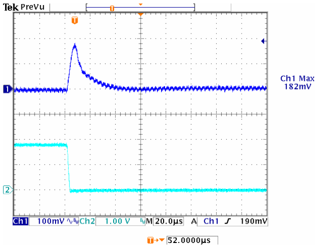
Figure 21: Typical Transient Response to Step Load Change at 2.5A/µS from 100% to 50% of I_o , max at 5Vin, 1.8Vout (Cout = 1µF ceramic, 10µF Tantalum)
