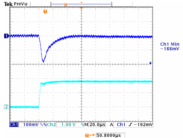
Figure 22: Typical Transient Response to Step Load Change at 2.5A/µS from 50% to 100% of I_o , max at 5Vin, 1.8Vout (Cout = 1µF ceramic, 10µF Tantalum)
