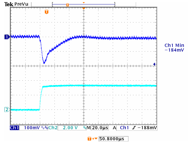
Figure 20: Typical Transient Response to Step Load Change at 2.5A/µS from 50% to 100% of I_o , max at 5Vin, 3.3Vout (Cout = 1µF ceramic, 10µF Tantalum)
