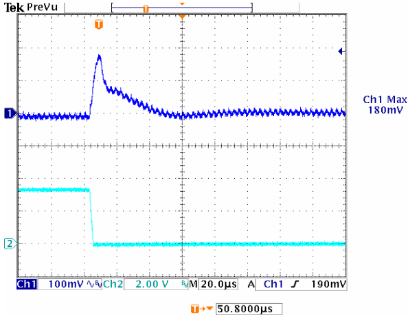
Figure 19: Typical Transient Response to Step Load Change at 2.5A/µS from 100% to 50% of I_o , max at 5Vin, 3.3Vout (Cout = 1µF ceramic, 10µF Tantalum)
