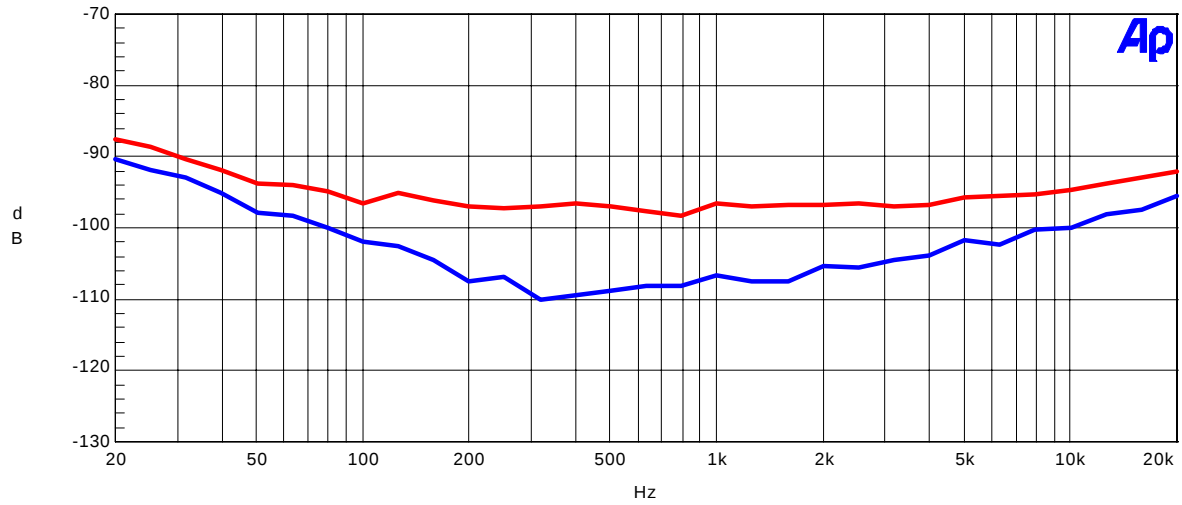
Fig5.Crosstalk
