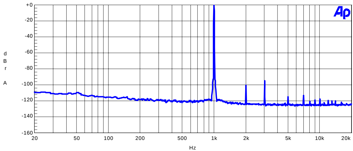
Fig6.FFT Plot
