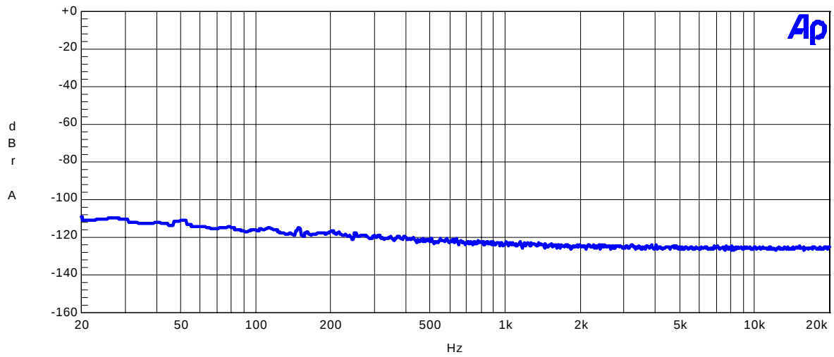
Fig 8. FFT Plot
