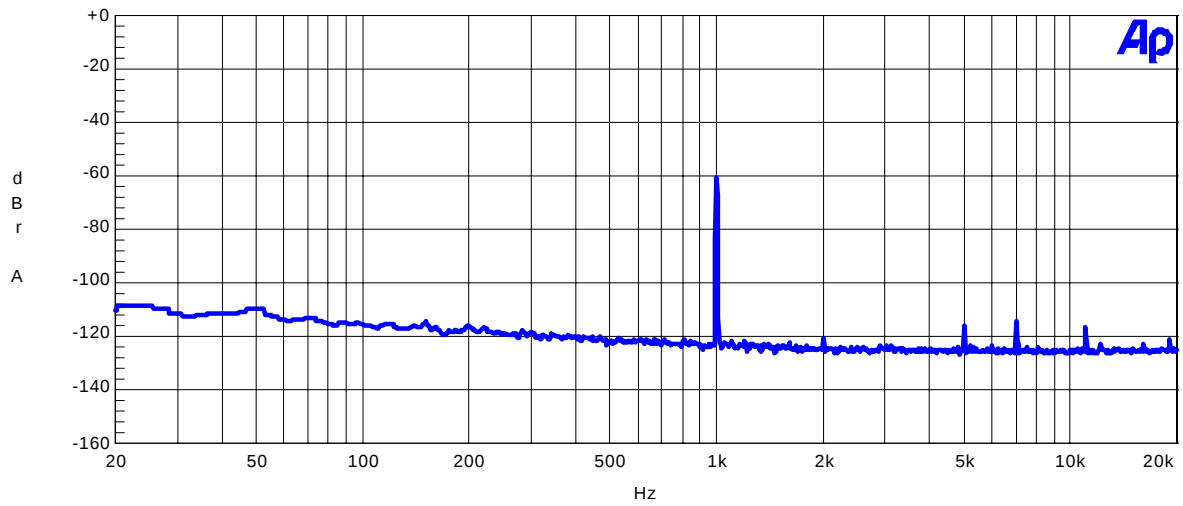
Fig 7. FFT Plot
