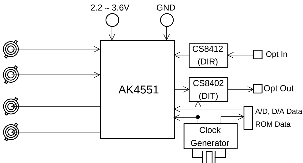
Figure 1. AKD4551 Block Diagram
