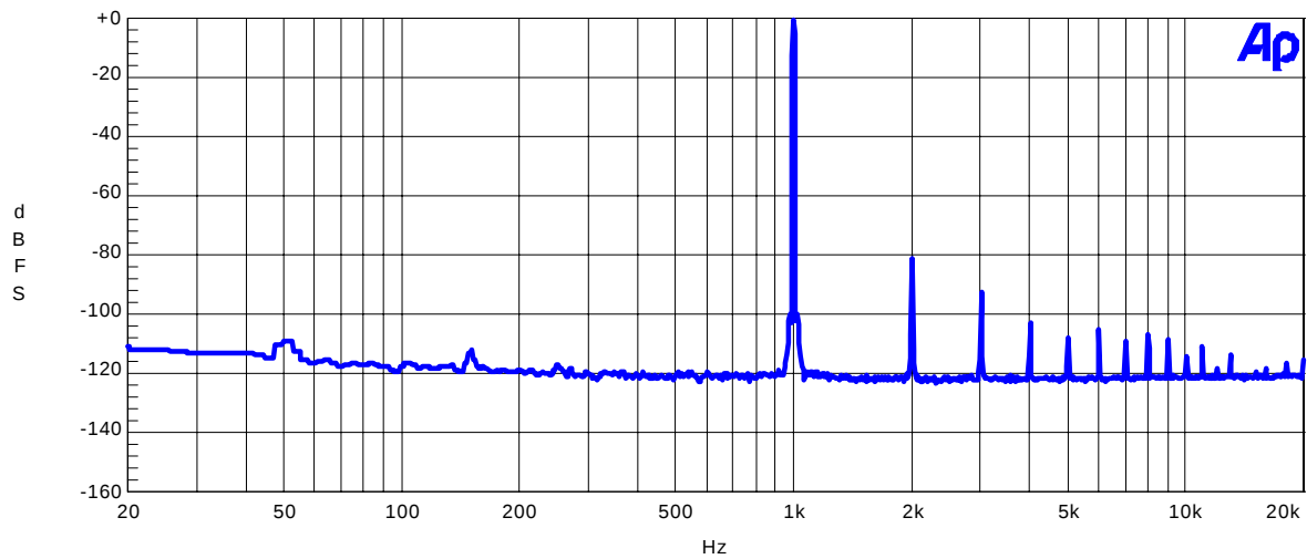
Fig6.FFT Plot
