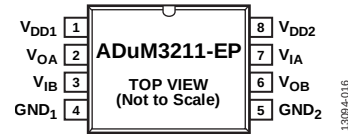
Figure 5. ADuM3211-EP Pin Configuration
