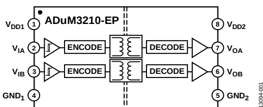
Figure 1. ADuM3210-EP Functional Block Diagram
