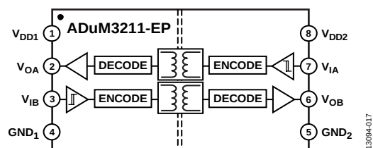
Figure 2. ADuM3211-EP Functional Block Diagram
