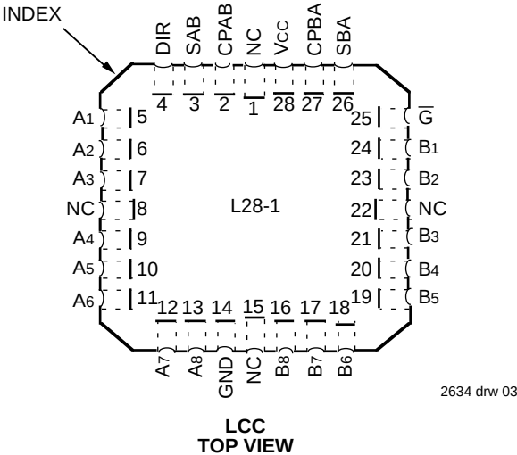
FCT646/FCT2646T FCT648
