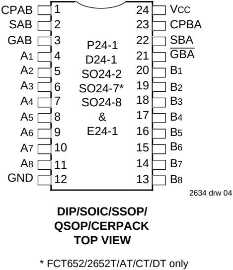
FCT652/FCT2652T
