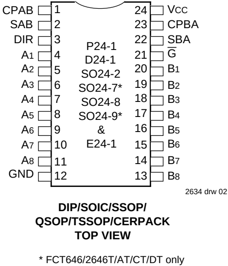
FCT646/FCT2646T FCT648
