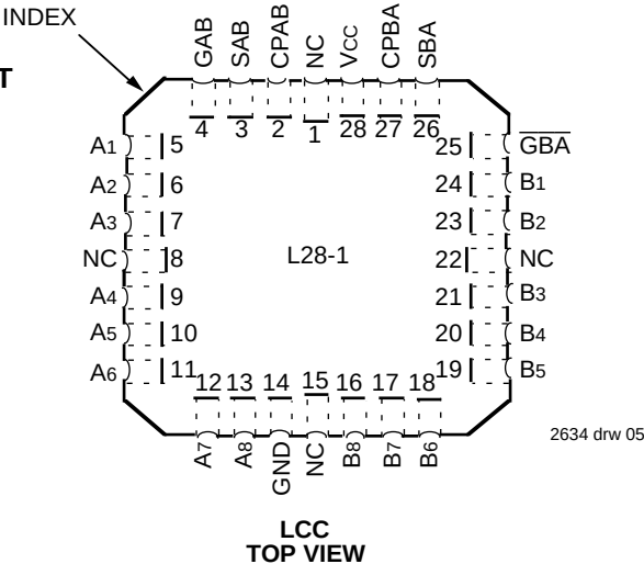
FCT652/FCT2652T
