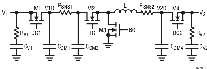
Figure 17. Power Path Capacitor Selection at V_1 and V_2
