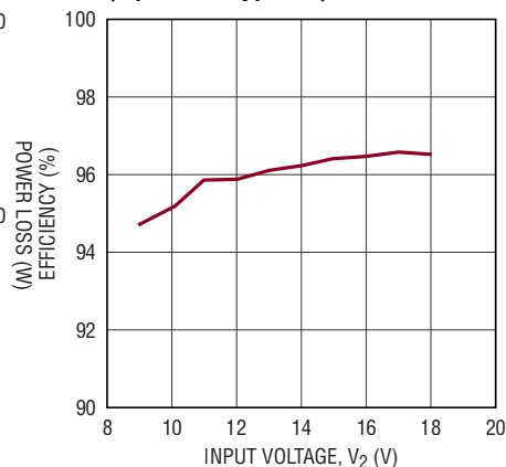
Efficiency vs V_2 (Boost) ( V_1 = 48\text{V} , I_{V1} = 5\text{A} )
