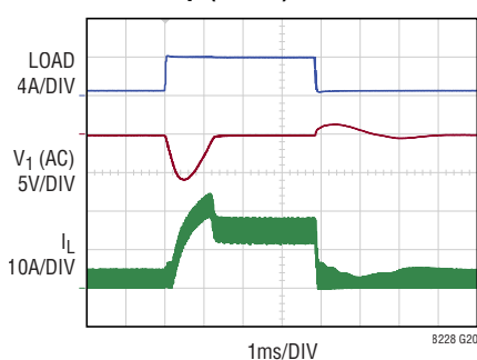
Load Step (Boost)
