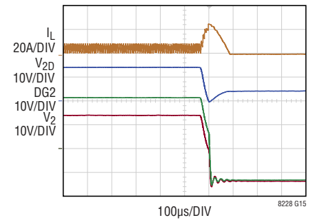
Reverse Battery Insertion at V_2 in Regulation
