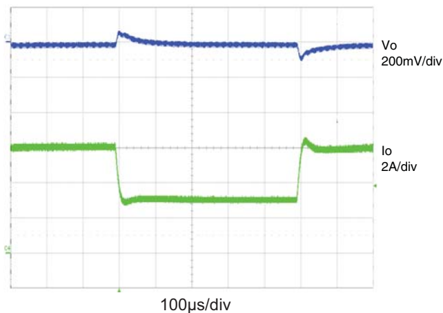
3A to 6A Load Transient
