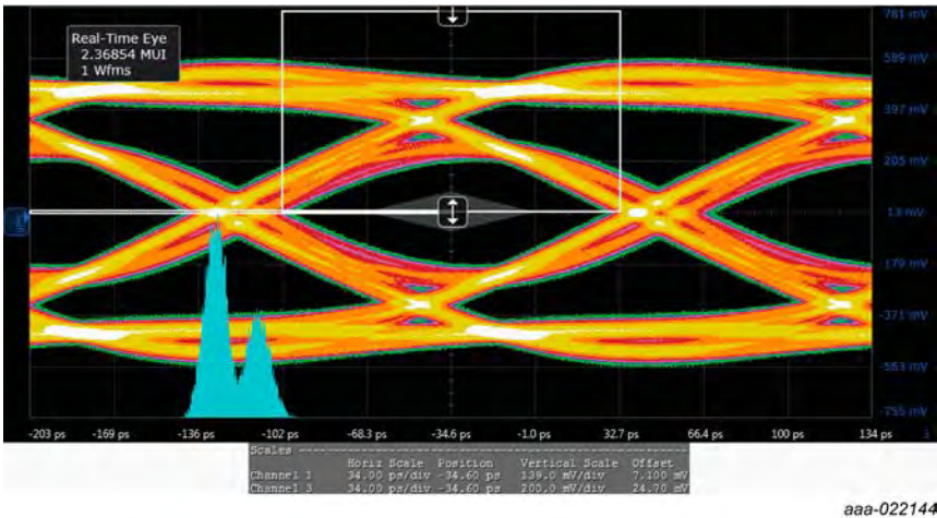
Fig 7. HDMI 2.0 eye diagram TP2, test board with PCMF2HDMI2S; typical values
