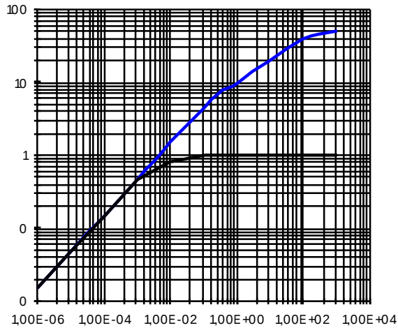
Figure 12 - Transient Thermal Imped. ( ^{\circ}\text{C}/\text{W} ) Vs Time (S)
