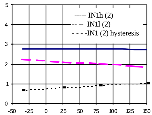
Figure 7 - IN1 & IN1h (2) thresholds (V) Vs T_j ( ^{\circ}\text{C} )
