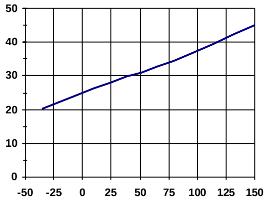
Figure 6 - IN1 (2) current ( \mu\text{A} ) Vs T_j ( ^{\circ}\text{C} )
