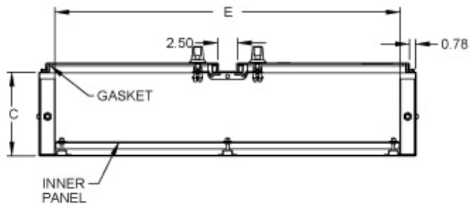
SECTION X-X
