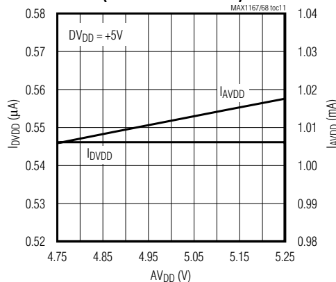
SHUTDOWN SUPPLY CURRENT vs. AV_{DD} SUPPLY VOLTAGE (EXTERNAL REFERENCE)
