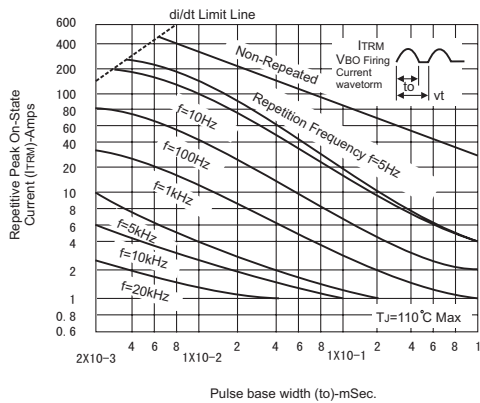
FIG.4 Repetitive Peak On-State Current (I TRM ) vs Pulse Width at Various Frequencies
