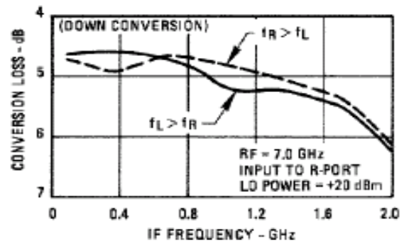
Conversion Loss
