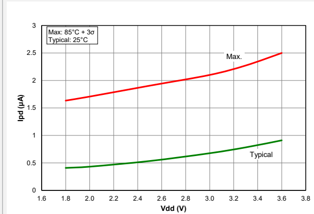
Figure 39-61. I_{PD} , Watchdog Timer, PIC18LF26/45/46K40 only
