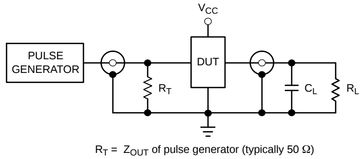
Figure 4. Test Circuit
