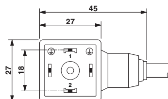
Dimensioned drawing
