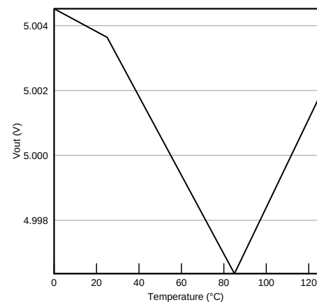
Figure 8. V_{OUT} vs Temperature
