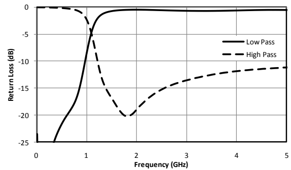
Fig. 3. Return loss.
