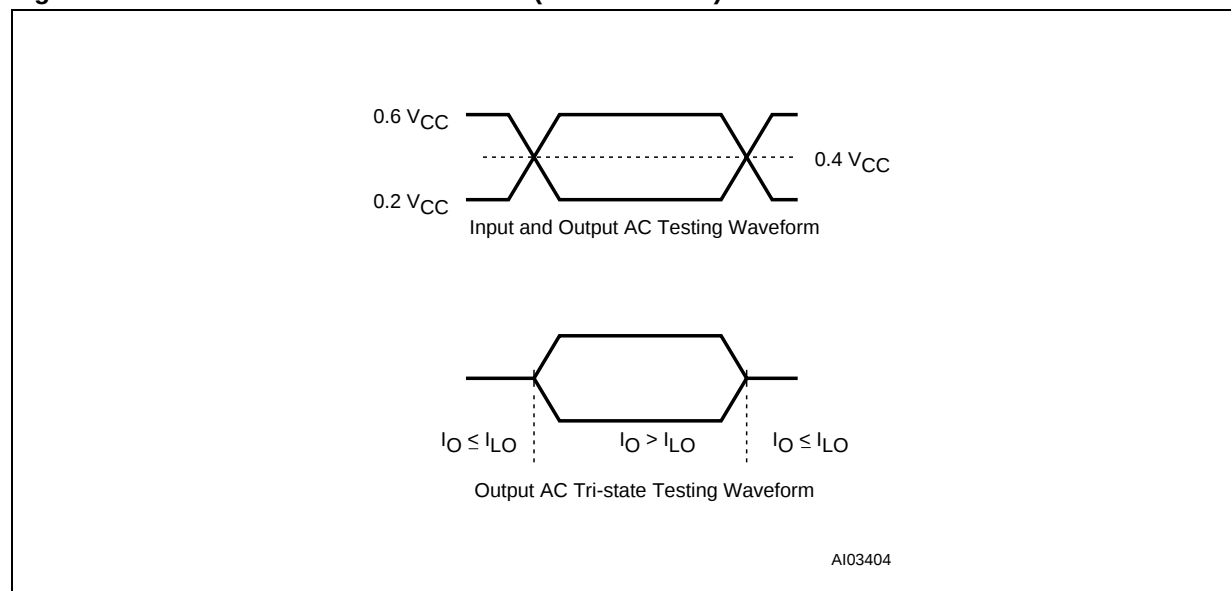
Figure 7. AC Measurement I/O Waveform (LPC Interface)
