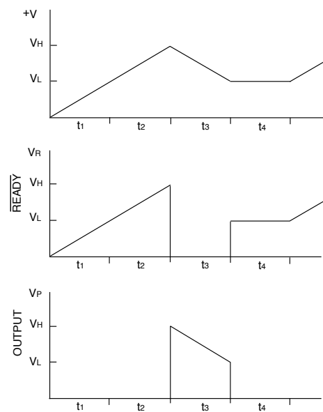
EH300/EH301 Waveforms
