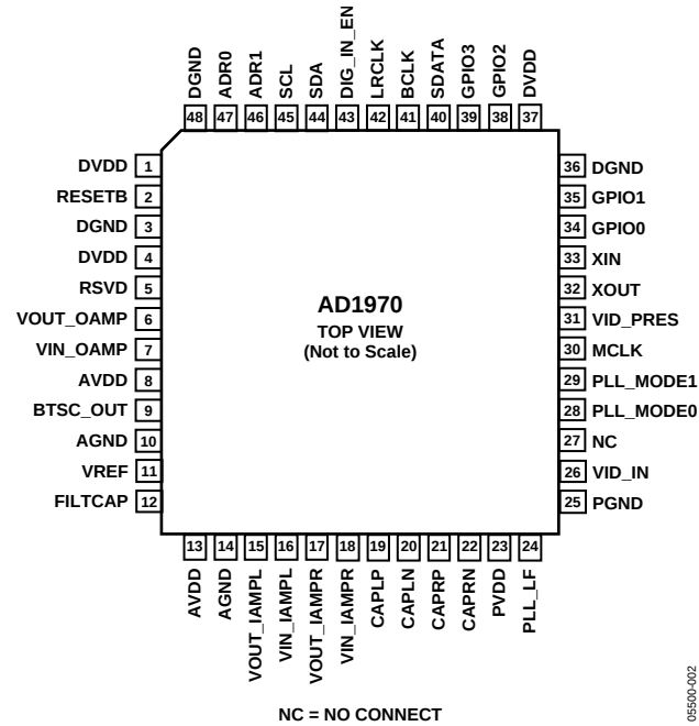
Figure 2. Pin Configuration
