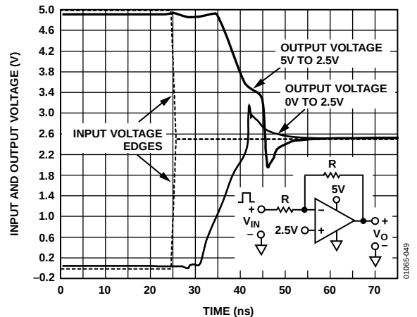
图49. 过载恢复( G = -1 , V_s = 5\text{ V} )
