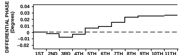
图23. 差分增益和相位误差 ( G = 2 , NTSC输入信号, R_L = 150\Omega , V_S = 5V )
