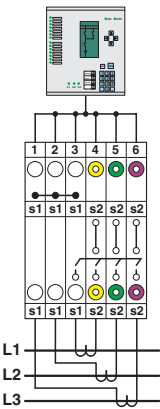
Interlinked three-phase current transformer set
