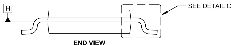
END VIEW
