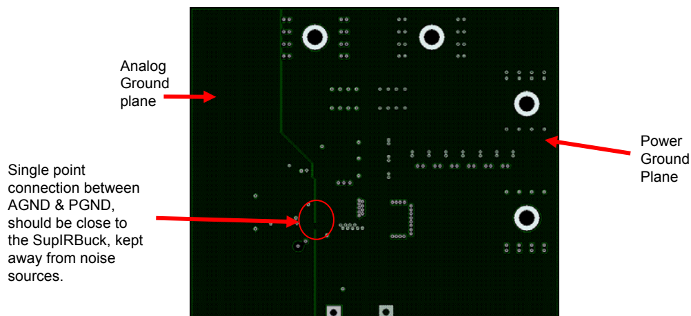
Fig. 26c. IRDC3842A demoboard layout considerations – Mid Layer 1
