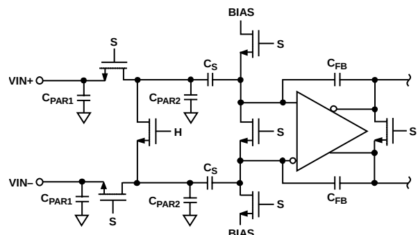
Figure 41. Switched Capacitor Input
