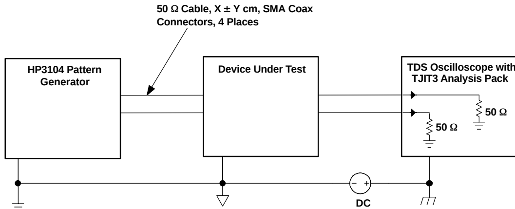
Figure 5. Jitter Measurement Setup
