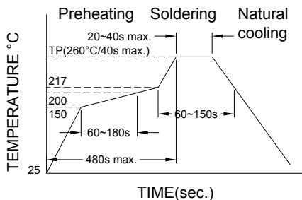
Figure 1. Re-flow Soldering
