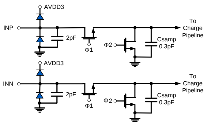
FIGURE 28. ANALOG INPUTS
