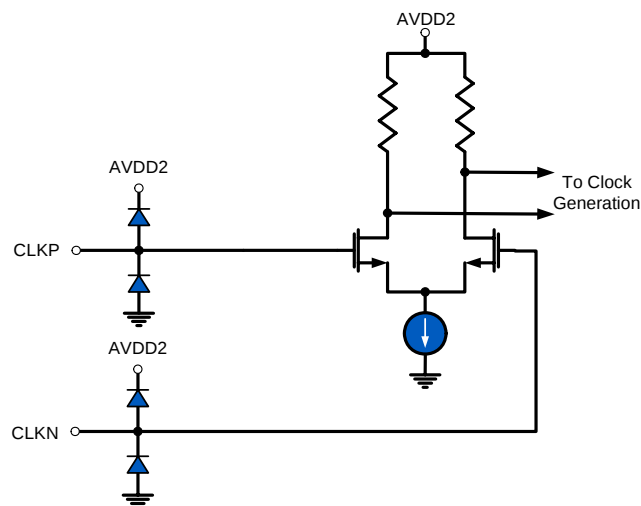
FIGURE 29. CLOCK INPUTS
