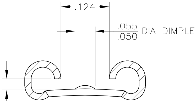
SECTION A-A SCALE 8:1
