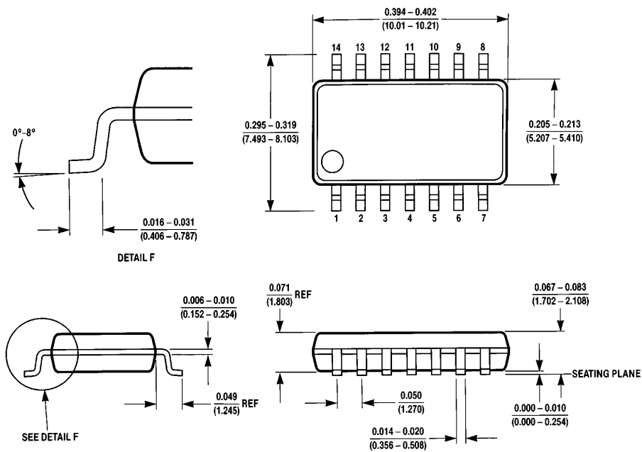
Small Outline Package (SJ) Order Number DM74ALS08SJ NS Package Number M14D
