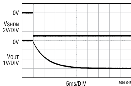
Fast \overline{SHDN} Start-Up
