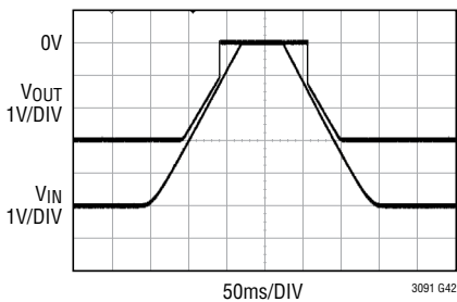
Slow Input Supply Ramp-Up and Ramp-Down
