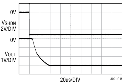
Fast \overline{SHDN} Start-Up
