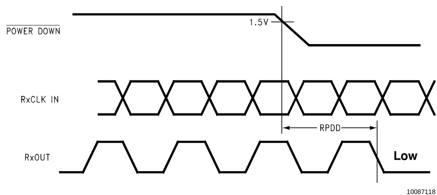
FIGURE 7. Receiver Powerdown Delay
