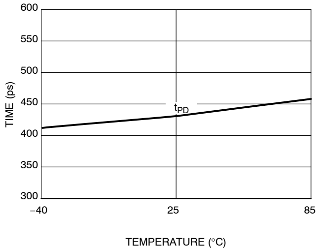
Figure 6. Typical Propagation Delay vs. Temperature ( V_{CC} - V_{EE} = 3.3 V; V_{TT} = 3.3 V @ 25°C; V_{in} = 100 mV; R_L = 50 \Omega )
