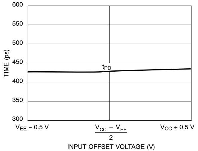
Figure 7. Typical Propagation Delay vs. Input Offset Voltage ( V_{CC} - V_{EE} = 3.3 V; V_{TT} = 3.3 V @ 25°C; V_{in} = 100 mV R_L = 50 \Omega )
