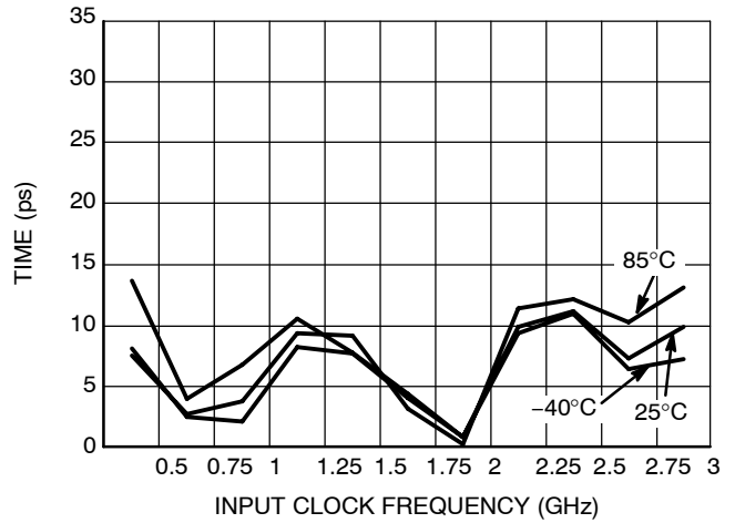
Figure 5. Data Dependent Jitter vs. Frequency and Temperature ( V_{CC} - V_{EE} = 3.3 V; V_{TT} = 3.3 V @ 25°C; V_{IN} = 100 mV; PRBS 2 23 -1; R_L = 25 \Omega )
