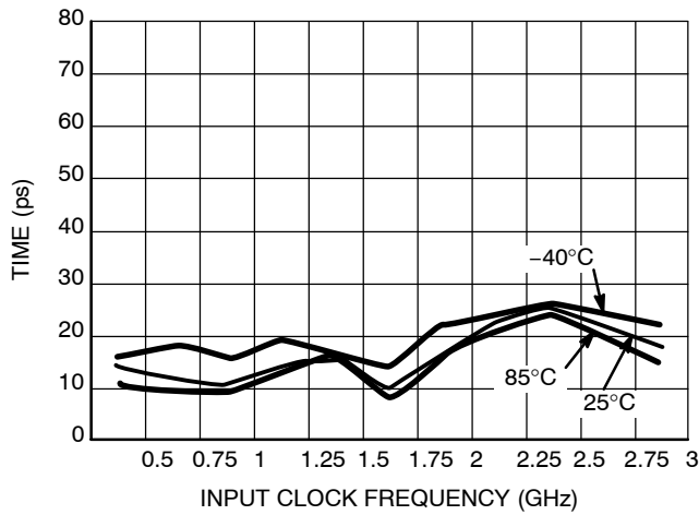
Figure 4. Data Dependent Jitter vs. Frequency and Temperature ( V_{CC} - V_{EE} = 3.3 V; V_{TT} = 3.3 V @ 25°C; V_{IN} = 100 mV; PRBS 2 23 -1; R_L = 50 \Omega )
