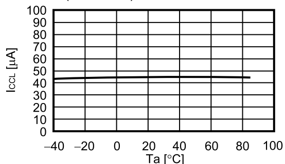
I_{CCL} vs. T_a ( V_{IN} = 3.3\text{ V} )
