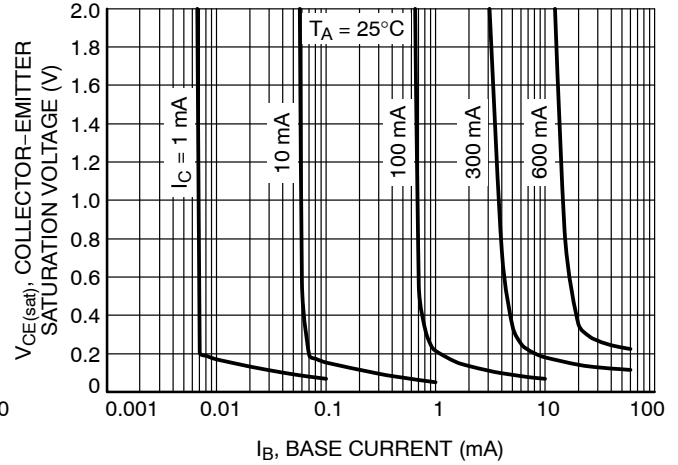
Figure 6. Saturation Region
