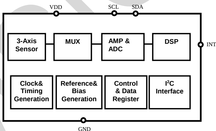
Figure 1: MXC6655XA Functional block diagram
