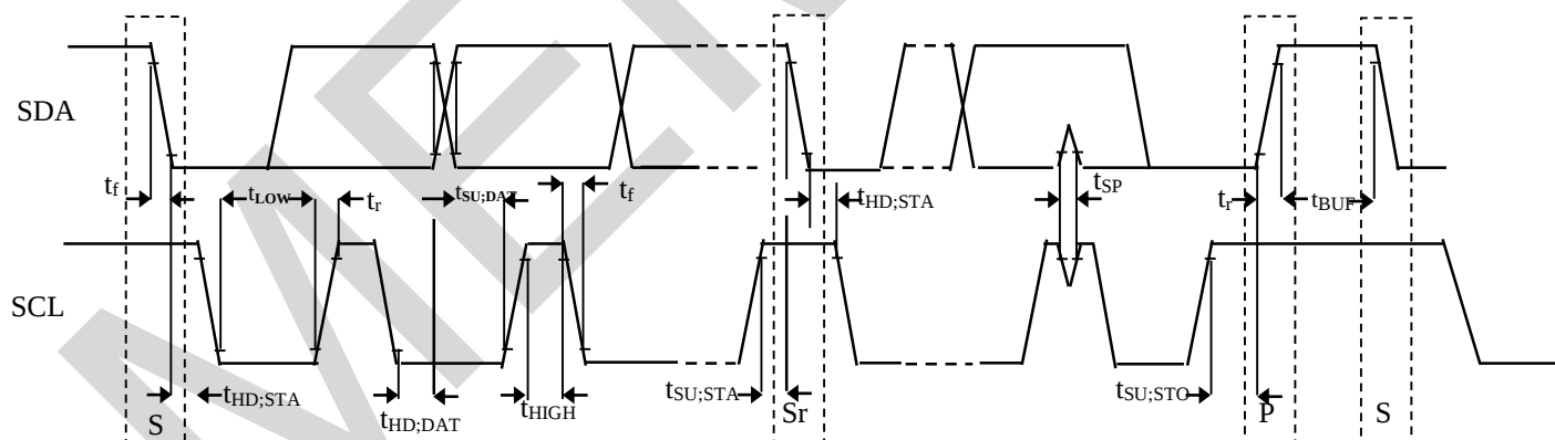
Figure 7: I 2 C timing
