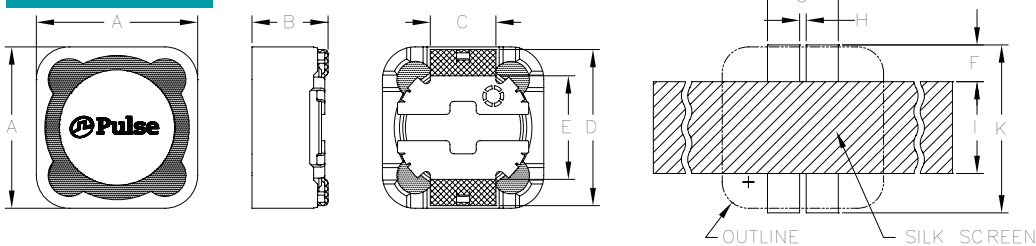
FINAL OUTLINE
