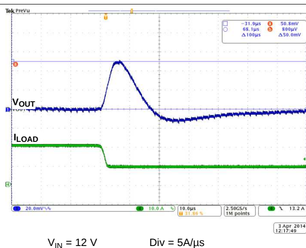
Figure 29. Load Step 20 A to 10 A
