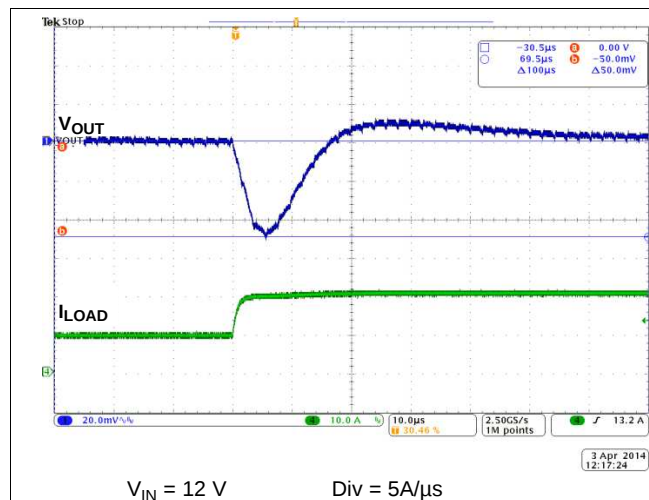
Figure 28. Load Step 10 A to 20 A
