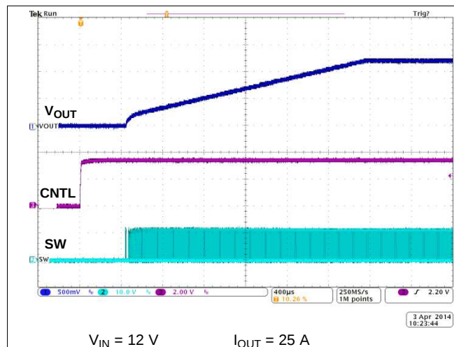
Figure 26. Startup from CNTL
