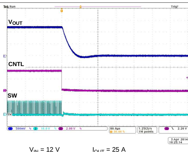
Figure 27. Shutdown from CNTL
