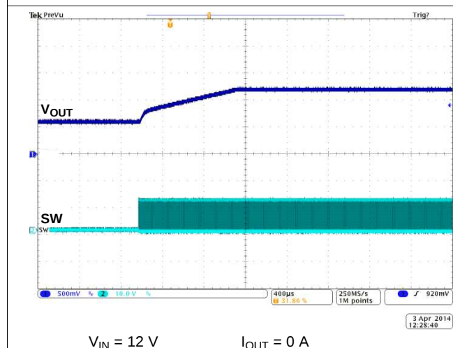
Figure 30. Prebias Sequence
