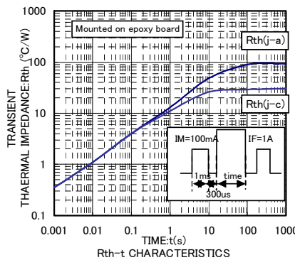
Rth-t CHARACTERISTICS
