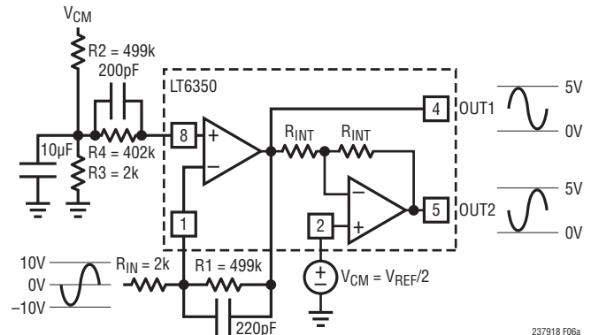
Figure 6a. LT6350 Converting a \pm 10\text{V} Single-Ended Signal to a \pm 5\text{V} Differential Input Signal
