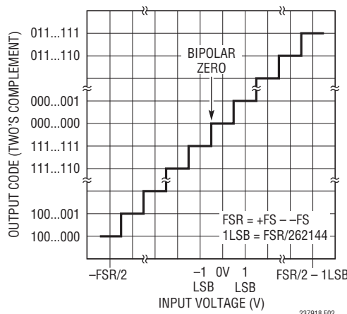
Figure 2. LTC2379-18 Transfer Function
