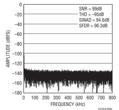
Figure 9b. 32k Point FFT Plot with f_N = 2\text{kHz} for Circuit Shown in Figure 9a
