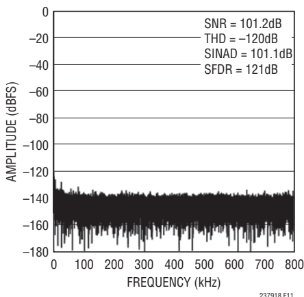
Figure 11. 32k Point FFT of the LTC2379-18
