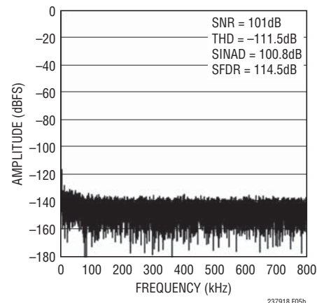
Figure 5b. 32k Point FFT Plot with f_{IN} = 10\text{kHz} for Circuit Shown in Figure 5a
