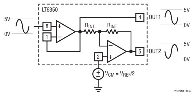
Figure 5a. LT6350 Converting a 0V-5V Single-Ended Signal to a \pm 5\text{V} Differential Input Signal
