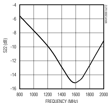
AMP 1 S_{22}
