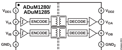
Figure 1. ADuM1280/ADuM1285
