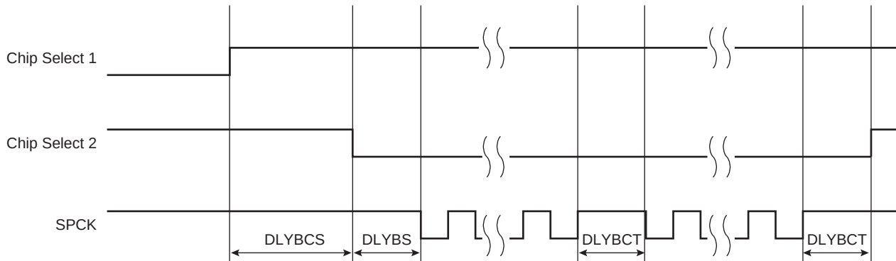
Figure 33-10. Programmable Delays
